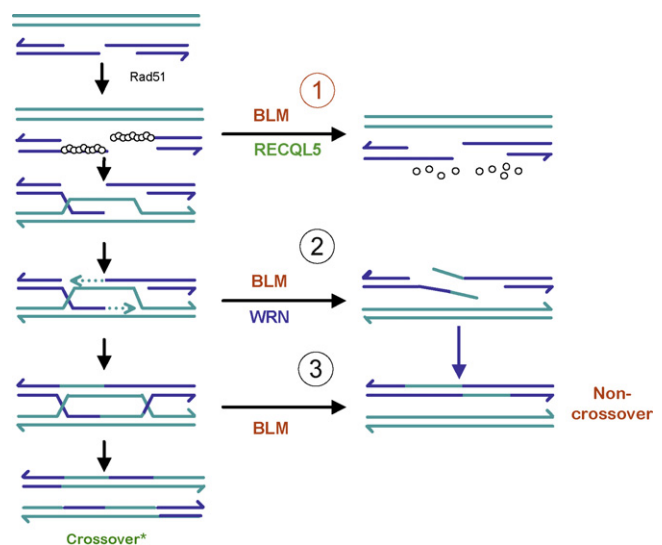
Fig. 1. Proposed pro- and anti-recombinogenic roles for BLM, WRN, and RECQL5. In step 1, BLM and RECQL5 disrupt the RAD51-ssDNA filament. In steps 2 and 3, BLM and WRN promote non-crossover resolution of recombination intermediates, including the double Holliday intermediate. BLM is the only RecQ helicase capable of promoting dissolution of a double Holliday junction. *Only one of the two possible crossover products is shown.
